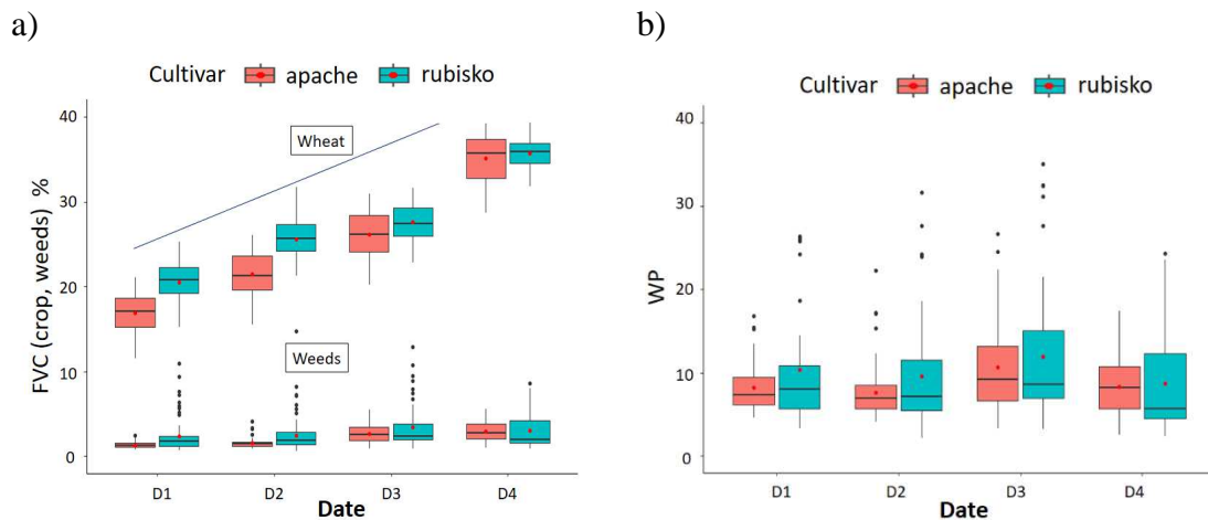
Figure 3. Temporal evolution of a) FVCc and FVCw and b) weed pressure indicator (WPI) for both the Apache and Rubisko cultivars.
