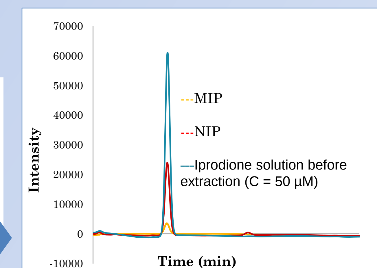
Fig. 1 : iprodione chromatograms superposition before and after extraction by MIP5 and NIP5 (methacrylamide, TRIM, precipitation).
