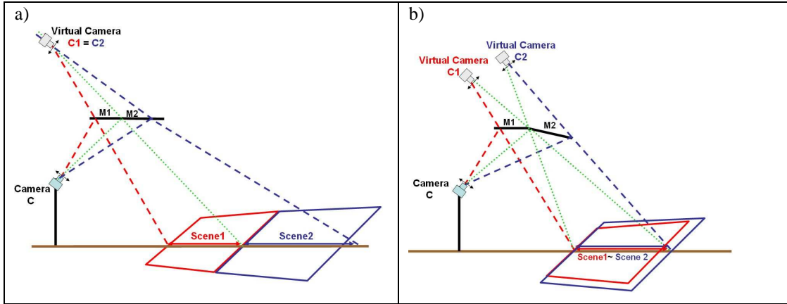
Fig. 2. a) General view of a bi-spectral imaging system based on a single camera (C) with 2 mirrors (M1 and M2). b) Superimposition of the two scenes for particular angles of mirrors (M1 and M2).
