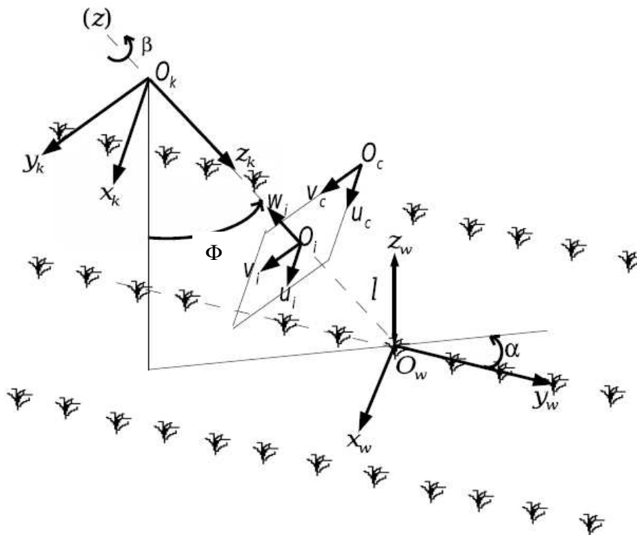
Fig. A1. Optical system with different coordinate systems : camera , image and real world.
