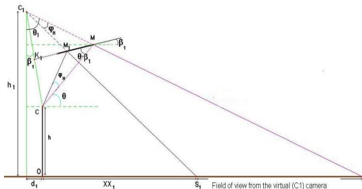
Fig. 1. a) The catadioptric viewer composed of a CCD monochrome camera with 2 mirrors placed above the camera. An interferential filter is fixed on each mirror. b) Optical model of the viewer system considering only one mirror (M1).
