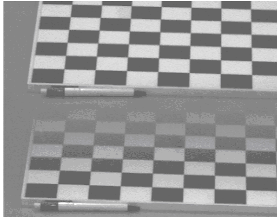
Fig. 3. A pair of images splitted vertically from the vision system composed of a CCD monochrome camera with 2 mirrors placed above the camera.
