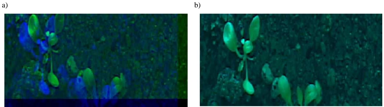
Fig.5: a) Superimposition of a pair of rectified images which have been splitted vertically from the vision system composed of a CCD monochrome camera with 2 mirrors (Green color : image from M1 and Blue color : image from M2). b) Correction with a vertical offset (13pixels) and an horizontal offset (15pixels).
