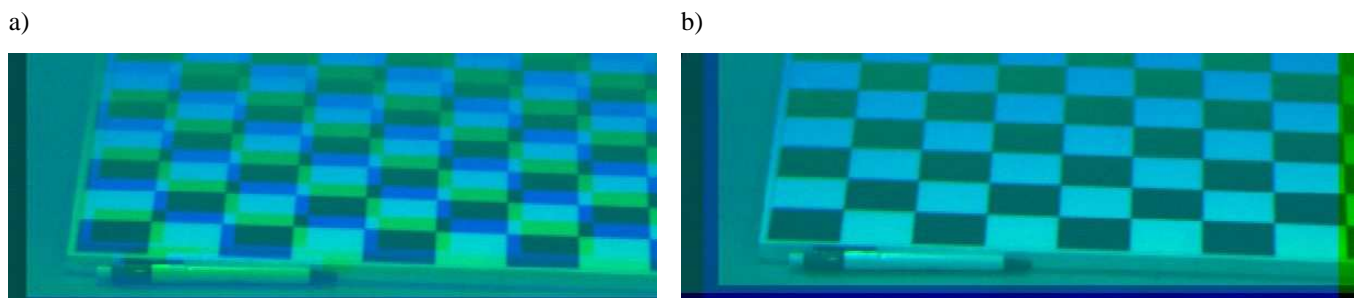
Fig.4: a) Superimposition of a pair of images splitted vertically from the vision system composed of a CCD monochrome camera with 2 mirrors (Green color: image from M1 and Blue color: image from M2) placed above the camera. b) Correction of a vertical offset (13pixels) and an horizontal offset (15pixels).
