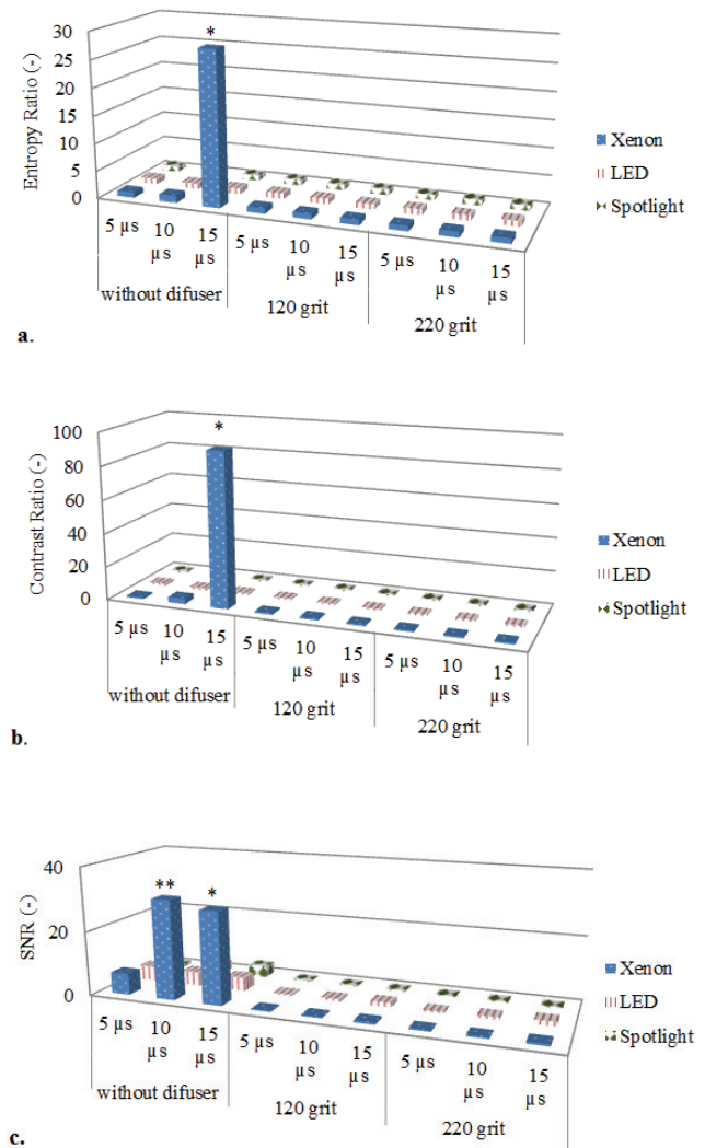
Figure 6. Image quality parameters (a) entropy ratio, (b) contrast ratio, and (c) SNR for the macro video zoom lens for different exposure times and lighting systems. Bars with asterisks are statistically different: * = p < 0.05 (Scheffé test) and ** = p < 0.05 (SNK test).
