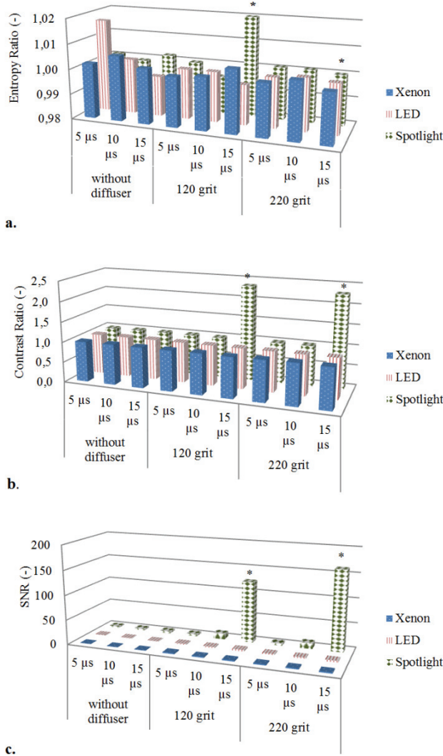
Figure 5. Image quality parameters (a) entropy ratio, (b) contrast ratio, and (c) SNR for the macro video zoom lens for different exposure times and lighting systems. Bars with asterisks are statistically different: * = p < 0.05 (Scheffé test).
