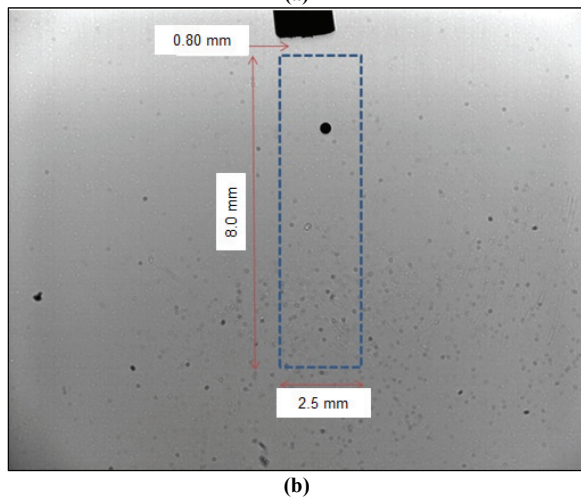
Figure 4. Region of interest (ROI) (blue dotted rectangle): (a) with the macro video zoom lens and xenon light with 120 grit diffuser at 15 \mu s exposure time, and (b) with the K2/SC long-distance microscope lens and xenon light without a diffuser at 5 \mu s exposure time.
