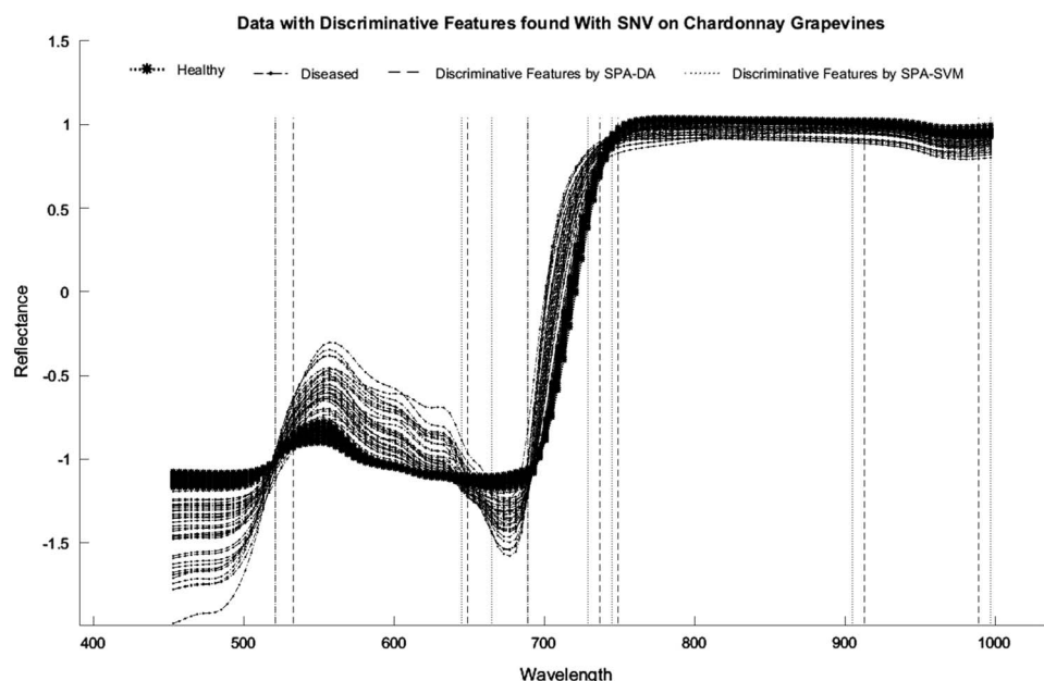
Figure 5 Chosen wavelengths (nm) by DA and SVM classification on variables selected with SNV pre-processing.
