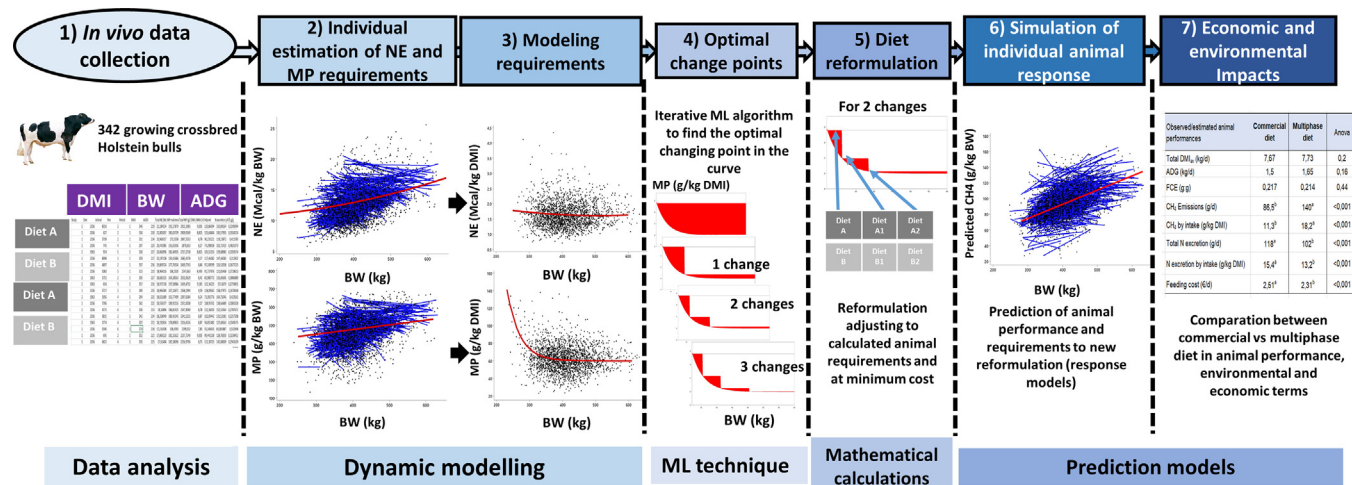
Fig. 1. Methodological steps followed in this work to simulate the impacts of a multiphase vs. commercial diet on crossbred Holstein bulls during fattening period. Abbreviations: DMI = DM intake, ADG = average daily gain, NE = net energy, MP = metabolisable protein, ML = machine learning, FCE = Feed conversion efficiency, CH 4 = enteric methane, N = Nitrogen.
