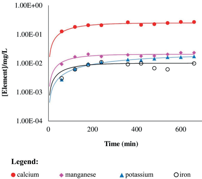
FIGURE 6. Refinement with an Avrami law: C(t) = C_{max} (1 - e^{-k t^n}) of the dissolution of calcium, manganese, potassium and iron during the first 12 hours of contact with a model wine. The concentrations are reported for 1 mg of ceramic.
