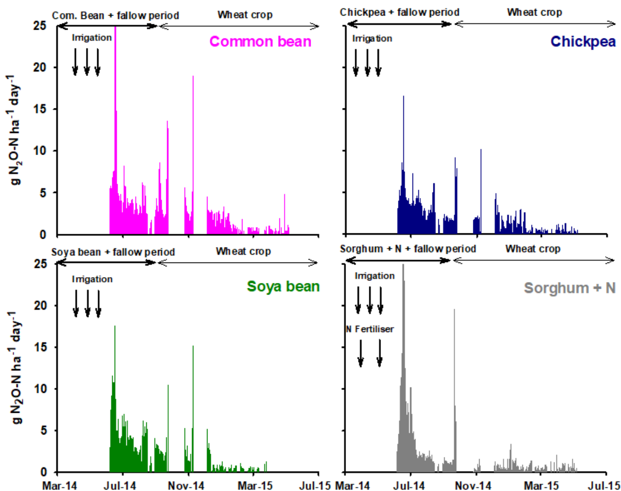
Figure 2 Daily N 2 O emissions for crops sown in May and for experiment A (2014-2015). Pre-crops are common bean, chickpea soya bean and sorghum. Measurements were performed 4 times a day. Amounts of N fertilizer (for sorghum) and irrigated water (for all crops) are given in part 2.2.
