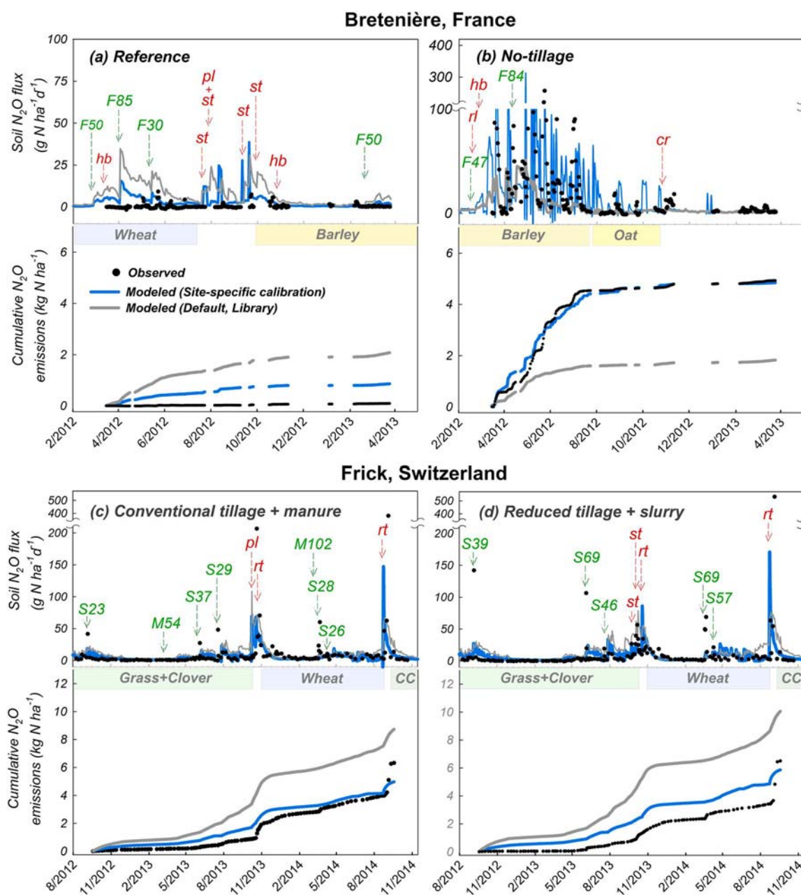
Fig. 3. Modeled (lines) versus observed (symbols) daily soil N 2 O fluxes (top panels) and cumulative N 2 O emissions (lower panels) from the ‘Reference’ (a) and the ‘No-tillage’ (b) treatments in Bretenièrre (France) and from the ‘Conventional tillage + manure’ (c) and the ‘Reduced tillage + slurry’ (d) treatments in Frick (Switzerland). Arrows associated with lowercase letters indicate cultivation events ( cr = cover crushing, hb = herbicide, pl = moldboard plowing, rl = rolling, rt = rotary tillage, st = shallow tillage). Arrows associated with uppercase letters followed by values indicate N inputs, including fertilization type ( F = synthetic fertilizer, S = slurry, M = manure compost) and rates, in kg N ha -1 , respectively (e.g., F50 indicates an application of synthetic fertilizer at a rate of 50 kg N ha -1 ). Please note the scale and breaks in the Y-axis. The crop growing periods from sowing to harvest or termination are indicated below the X-axis of the upper panels. CC = cover crop.
