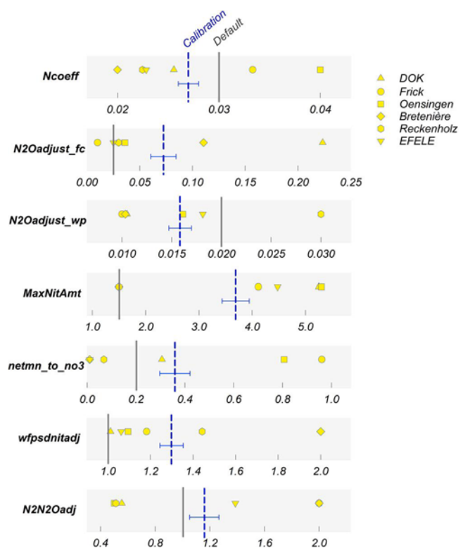
Fig. 6. DayCent parameters controlling soil N 2 O emissions before and after calibration based on data from six cropland field studies in Switzerland and France. The gray solid vertical lines indicate the original default model values of the parameter, the dashed blue lines indicate the value of the average calibration using all six sites with horizontal blue bars indicating the confidence interval of the leave-one-out values for \alpha = 0.05 . The yellow symbols indicate the values from the individual site-specific calibrations. Ncoeff = minimum water and temperature limitation coefficient for nitrification, N2Oadjust\_fc = maximum proportion of nitrified N lost as N 2 O at field capacity, N2Oadjust\_wp = minimum proportion of nitrified N lost as N 2 O at wilting point, MaxNitAmt = maximum daily nitrification amount (g N m -2 ), netmn\_to\_no3 = fraction of new net mineralization that goes to NO 3 , wfpsdnitadj = adjustment on inflection point for water-filled pore space effect on denitrification, N2N2Oadj = N 2 :N 2 O ratio adjustment coefficient.
