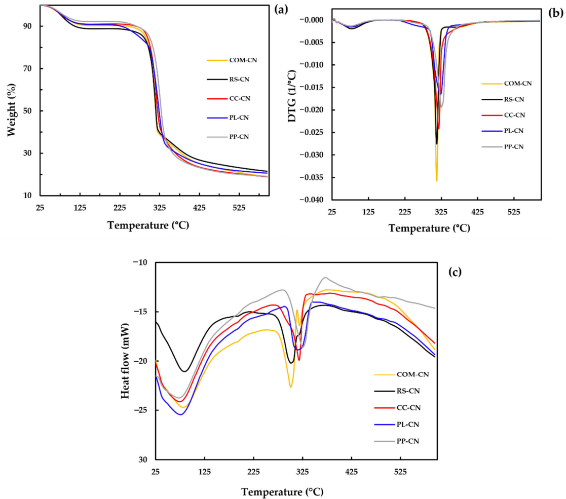
Figure 3. TGA (a), DTG (b), and DSC (c) curves of cellulose nanosphere isolated from different sources compared with commercial cellulose. RS-CN: rice straw cellulose nanosphere; CC-CN: corncob cellulose nanosphere; PL-CN: pineapple leaves cellulose nanosphere; PP-CN: pineapple peels cellulose nanosphere; COM-CN: cellulose nanosphere hydrolyzed from commercial cellulose.
