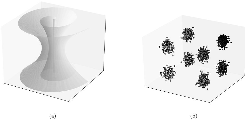
Figure 1: Figure 1a shows a surface in shades of grey that depicts an hourglass-shaped Swiss roll, as an instance of a two-dimensional subspace embedded in our usual three-dimensional space. Figure 1b presents eight dense clusters, separated by large empty regions in the three-dimensional space.
