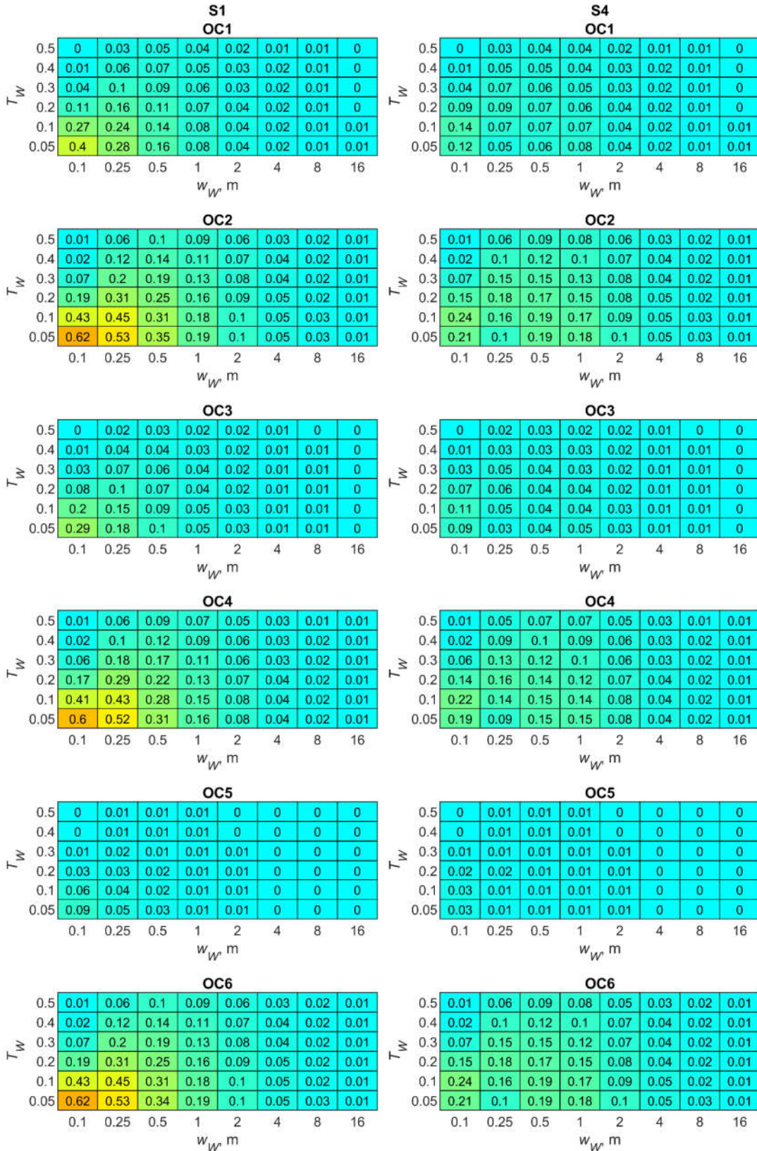
Fig. 6 - Matrices of values of T_{WA < 85\%} derived from spraying simulations for strategies S1 (left) and S4 (right), and for all the operating conditions (OC1 to OC6) with respect to weed patch width w_w and weed coverage rate T_w . To improve data readability, the matrix cells are coloured according to values (from blue (value 0) to red (value 1) in the web version or from white (value 0) to grey (value 1) in the printed version of this article).
