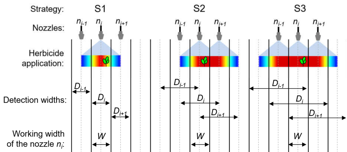
Fig. 2 - Illustration of the nozzle detection width defined for the three nozzle control strategies S1, S2 and S3. D_{i-1} , D_i and D_{i+1} are the detection widths associated with the nozzles n_{i-1} , n_i and n_{i+1} , while W is the working width.
