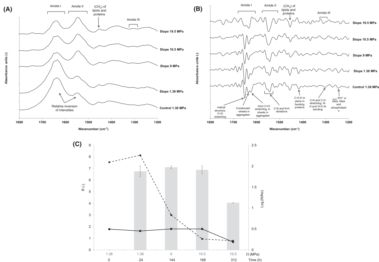
Fig. 4. FTIR spectra of S. cerevisiae grown at 1.38 MPa (control) or collected during a glycerol ramp in the spectral window of proteins (1200 to 1800 \text{cm}^{-1} ). During the ramp, cells were collected at 1.38, 9, 10.5 and 19.5 MPa.
