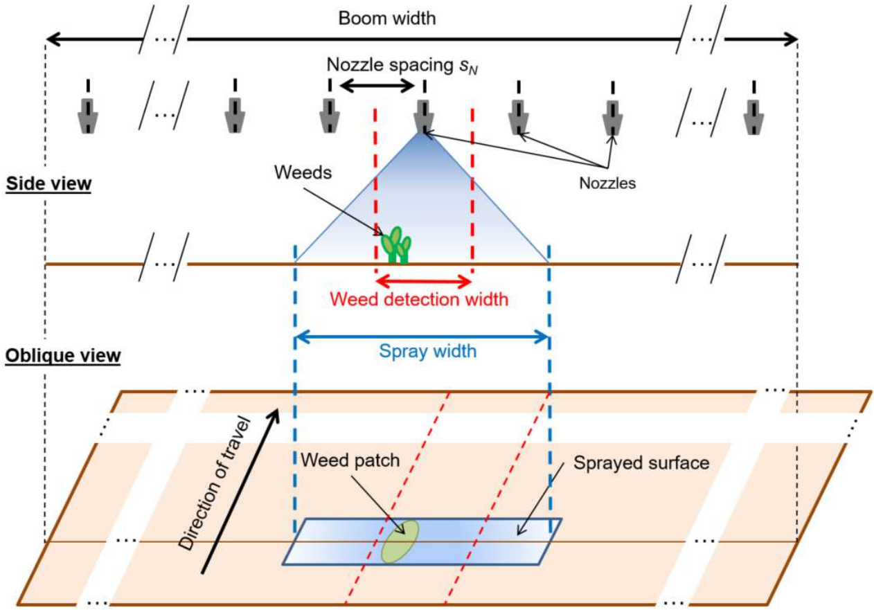
Fig. 4. Illustration of the weed detection width and the spray width in the case of nozzles controlled individually (only one nozzle is switched on in this example).
