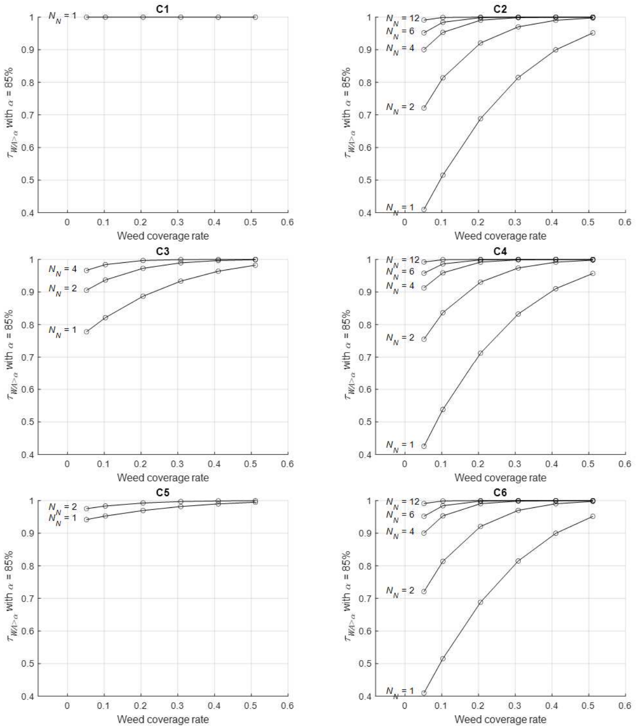
Fig. 9. Analysis of the weed area on which the application rate is higher than 85% ( \tau_{WA>85\%} ) with respect to the weed coverage rate, in the case of small patches ( l_e = 1 m, w_e = 0.2 m) and different operation conditions from C1 to C6 (Table 2). The section width (expressed in number of nozzles N_N ) is indicated on the left of the curves. The number of section widths presented on each graph was changed depending on the operating condition to improve readability and avoid curve overlay (for curves close to \tau_{WA>85\%} = 1 ).
