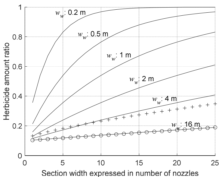
Fig. 10. Sprayed amount ratio computed for a weed coverage rate of 10% (continuous lines) and different patch width values ( w_w , indicated on the curves) with respect to the section width (expressed in number of nozzles spaced 0.5 m apart). Results derived from Franco et al. (2017) in the cases of scattered patches (+) and significant patches (○) are reproduced and superimposed.
