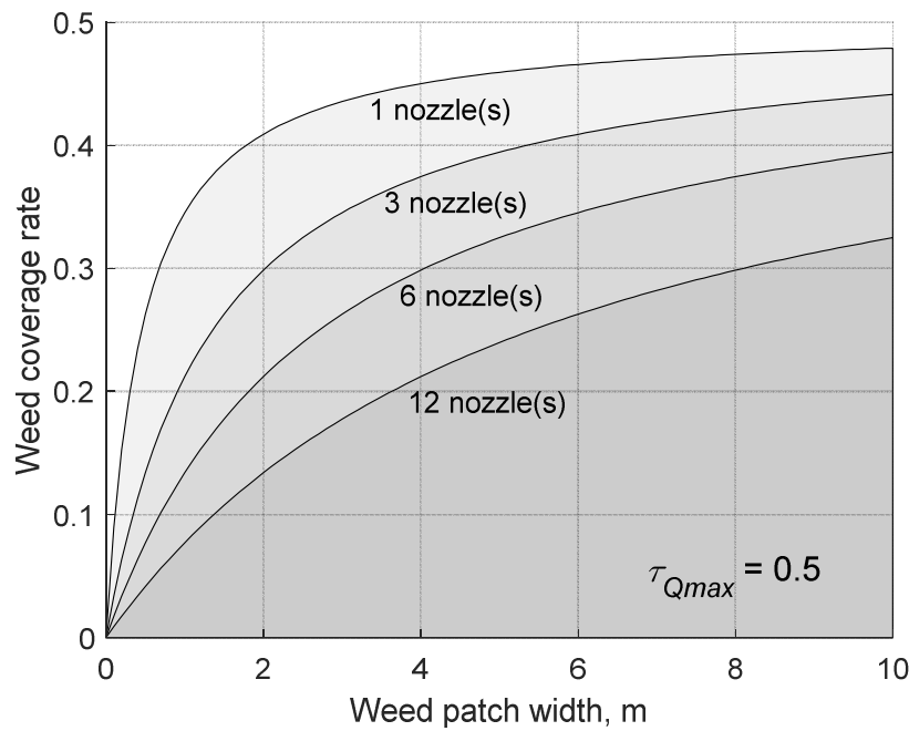
354 355 Fig. 7. Boom section width (expressed in number of nozzles spaced 0.5 m apart) required to reach an 356 herbicide amount reduction of 50%.
