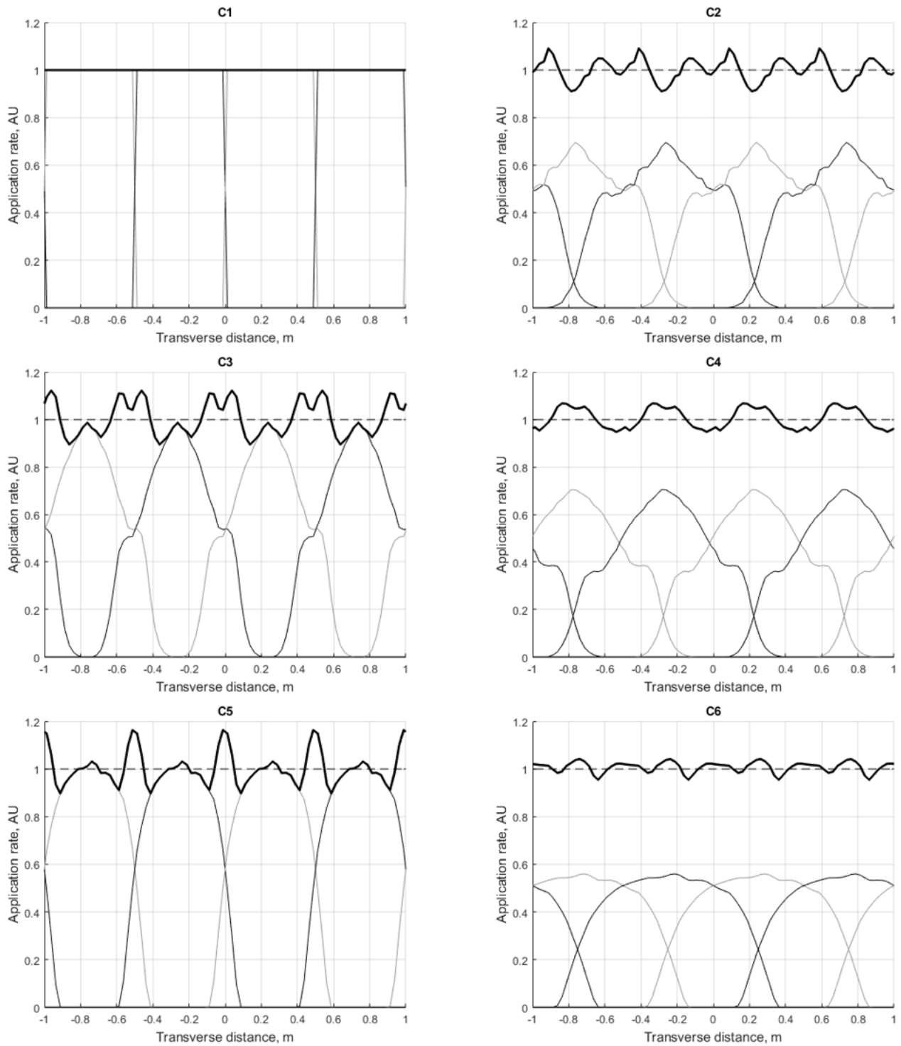
Fig. 3. Transverse spray patterns of adjoining single nozzles (thin lines alternatively grey or black for successive neighbouring nozzles) and global boom transverse spray patterns resulting from cumulated applications (bold line). The corresponding mean application rate (dotted line) along the boom is at the unit value (in Arbitrary Unit (AU)) for all operating conditions C1 to C6 (Table 2).
