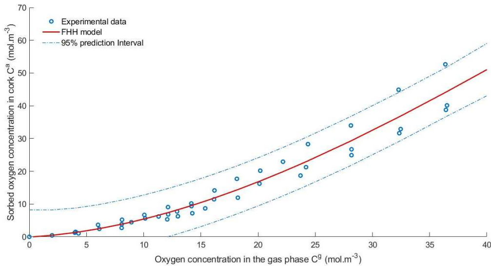
Figure 4: Sorption isotherm of oxygen on cork at 298 K for oxygen pressure ranging between 0 and 1000 hPa (o experimental data, - FHH model used to fit sorption data, -.- 95% prediction interval); (data from Lequin et al. 33 )
