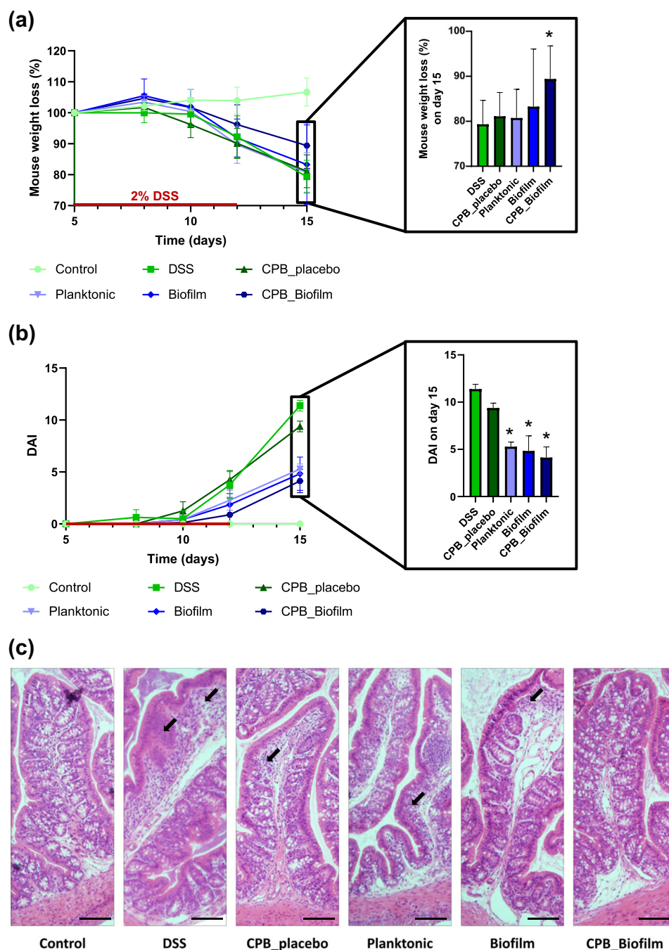
Fig. 5 Evaluation of treatment efficacy by biofilm-like L. paracasei ATCC334 encapsulated in pectin beads in DSS-induced colitis mice. The results presented are representative of 8 mice from each group. Asterisks indicate statistically significant differences from the DSS-induced colitic group (* P < 0.05 ), (Kruskal–Wallis test). a Changes in mouse body weight during and after DSS administration. The percent change in body weight was calculated by using the weight on day 5 (the day of DSS initiation) as the reference. b Clinical assessment of DSS-induced colitis. Disease Activity Index (DAI) was scored for each mouse for weight loss, stool consistency, and bleeding. c Histological sections of H&E-stained colon of representative mice from each group (tissue damage is shown by arrows) (scale bars, 30 µm).
