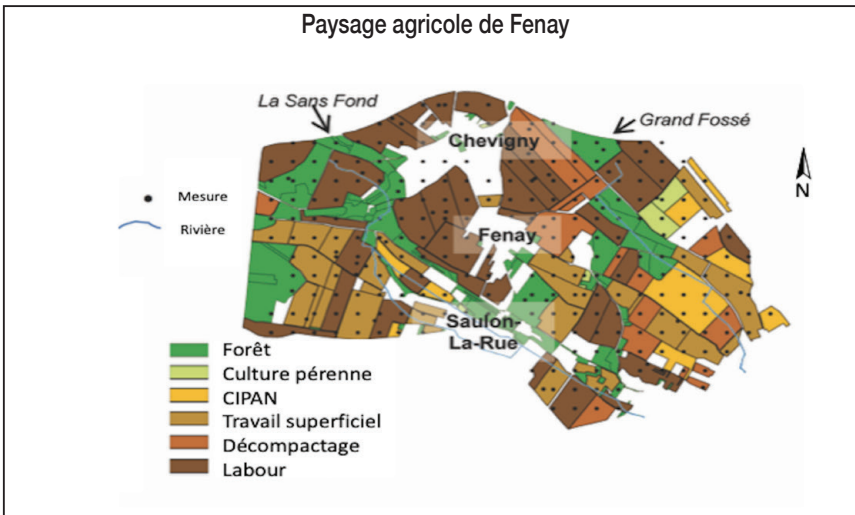
Figure 8 : Application des indicateurs microbiens sur le paysage agricole de Fenay. Figure 8: Application of microbial indicators on the agricultural landscape of Fenay.
