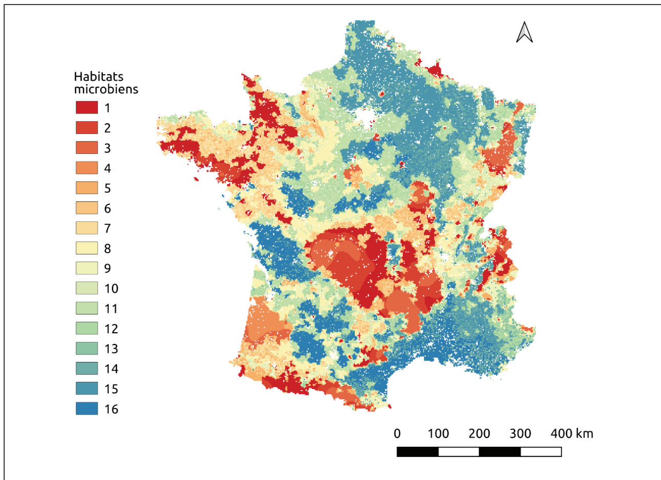
Figure 6: Mapping of microbial habitats at the scale of France.
