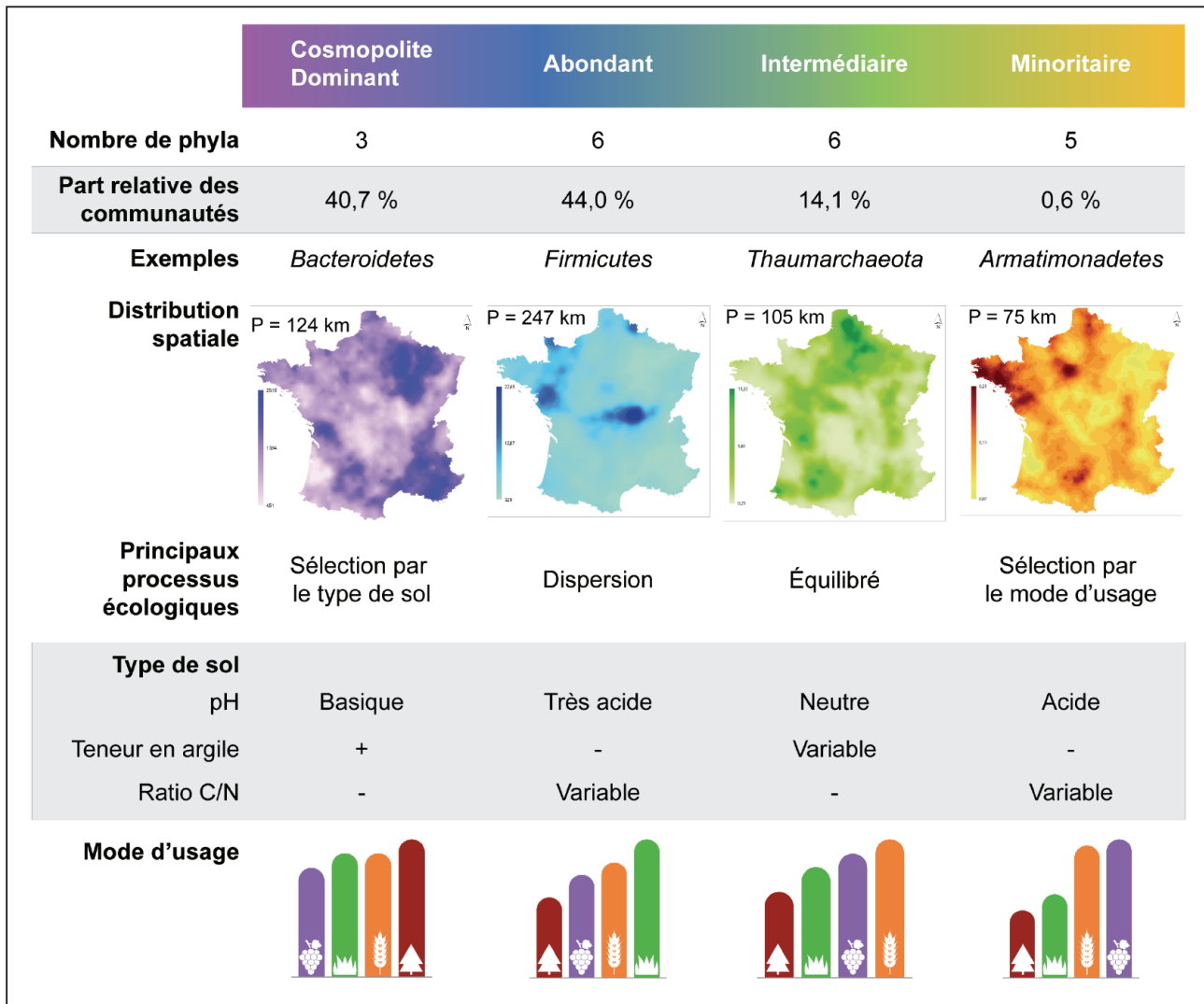
Figure 3: Distribution and ecological attributes of bacterial phyla at the scale of France.
