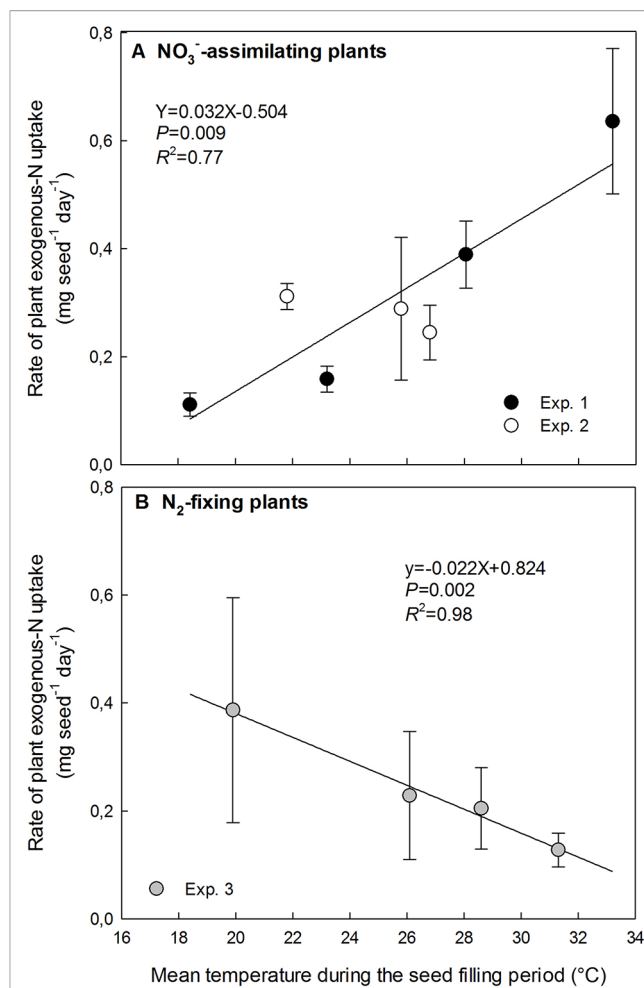
FIGURE 4 | Opposite responses to temperature increase of exogenous-N uptake rate in plants during the seed-filling period for \text{NO}_3^- -assimilating plants (A) and \text{N}_2 -fixing plants (B). The vertical bars represent SE. The data were fitted with a linear regression.
