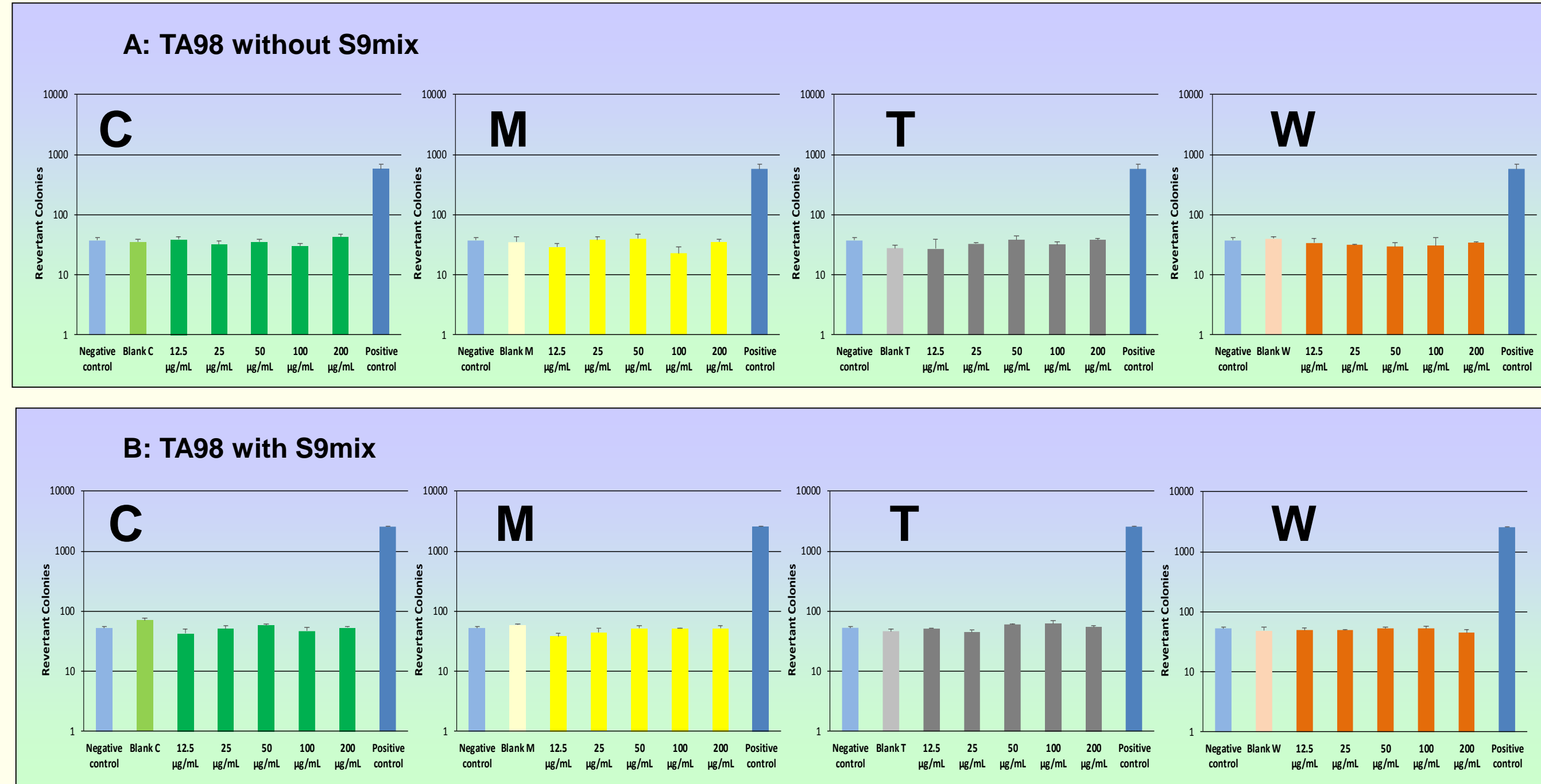
Figure 6: Number of revertant colonies measured in the Ames test on the TA98 strain in absence (A) and in presence (B) of S9 mix with 5 different concentrations (12.5 to 200 µg/mL) of Lebanese pita extracts (one independent experiment). Positive controls: 2-Nitrofluorene (2 µg/plate) without S9 mix, 2-Aminoanthracene (2.5 µg/plate) with S9 mix.
