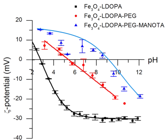
Figure 4. Zetametry of \text{Fe}_3\text{O}_4 -LDOPA, \text{Fe}_3\text{O}_4 -LDOPA-PEG, and \text{Fe}_3\text{O}_4 -LDOPA-PEG-MANOTA NPs.
