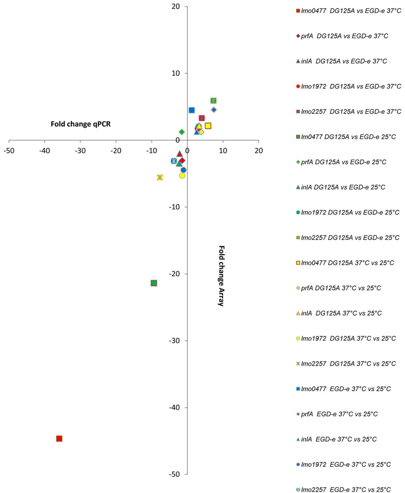
Figure 6. Comparison of fold-changes determined from microarray and reverse transcriptase real time PCR data. (□) Imo0477 , (◇) prfA , (Δ) inIA , (O) Imo1972 , (⊕) Imo2257 ; red : DG125A versus EGD-e 37°C, green : DG125A versus EGD-e 25°C, blue : EGD-e 37°C versus 25°C, yellow : DG125A 37°C versus 25°C. doi:10.1371/journal.pone.0043154.g006
