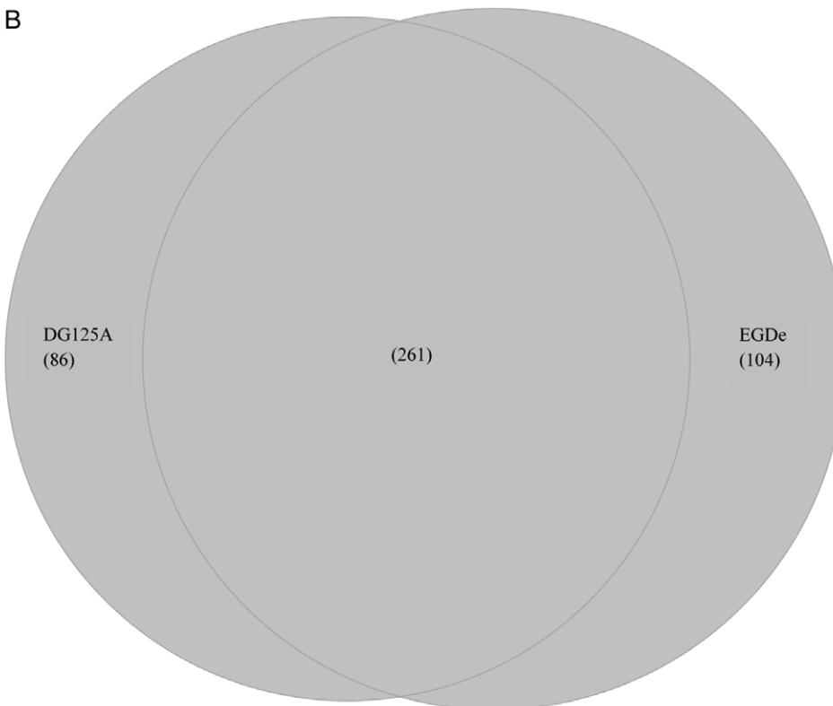
Figure 1. Venn diagrams of the overall number of genes with temperature-dependent variations and represented as specific or common to L. monocytogenes EGD-e and L. monocytogenes DG125A. (A) higher transcript levels at 25°C; (B) higher transcript levels at 37°C. doi:10.1371/journal.pone.0043154.g001
